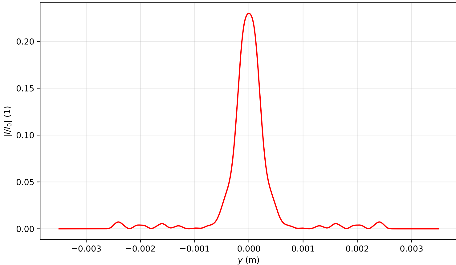
Intensity profile I(x=0, y, z=2.388)/I_0 , P_{in}=6.0P_{cr} , artificial time
